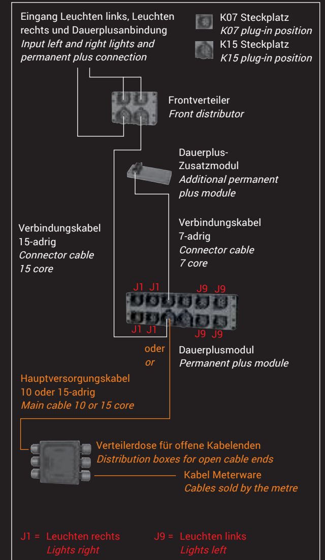
Uncontrolled Heckleuchten Zugfahrzeug Uncontrolled rear lights truck
