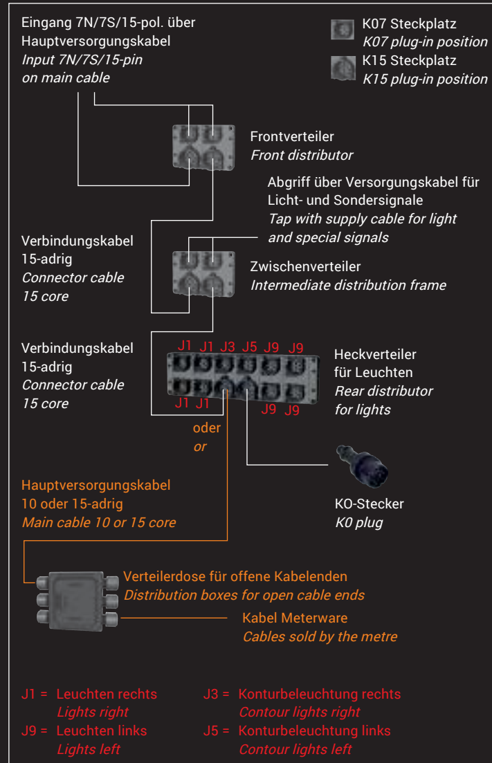
Controlled Heckleuchten Anhänger Controlled rear lights trailer
