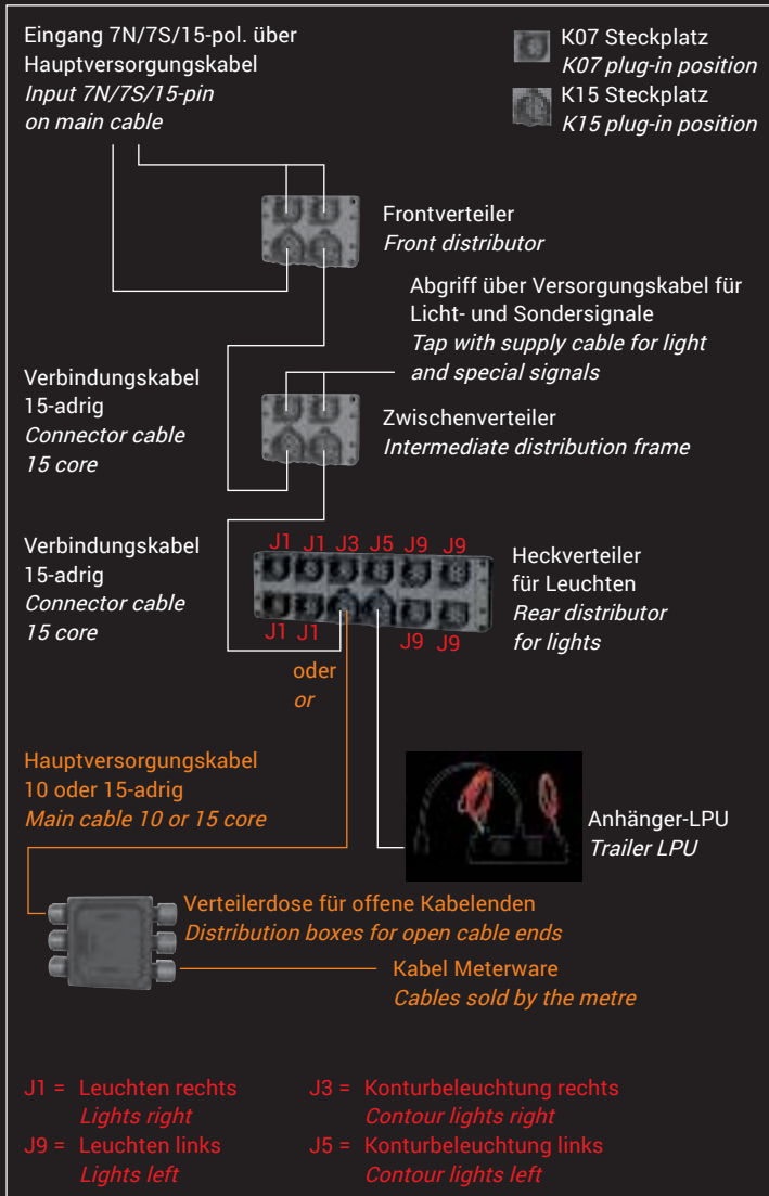
Uncontrolled Heckleuchten Anhänger Uncontrolled rear lights trailer
